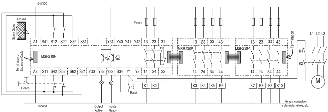
Dual Channel Safety Gate and E-Stop, Monitored Manual Reset, Monitored Output
