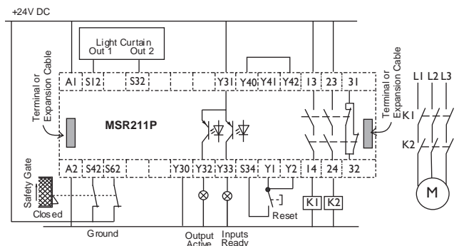
Light Curtain and Dual Channel Safety Gate, Monitored Manual Reset, No Monitored Output
