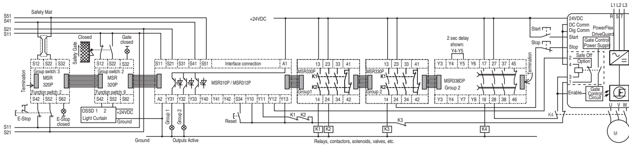
MSR 300 system with various Inputs. Two Output Groups with common monitored reset, each Group with monitored contactors Safety Mat or E-Stop shut down both Groups, Safety Gate and Light Curtain only shut down the Group 2 modules: Controlled Stop via instant contacts, delayed Safe Off and Power removal via MSR338DP
